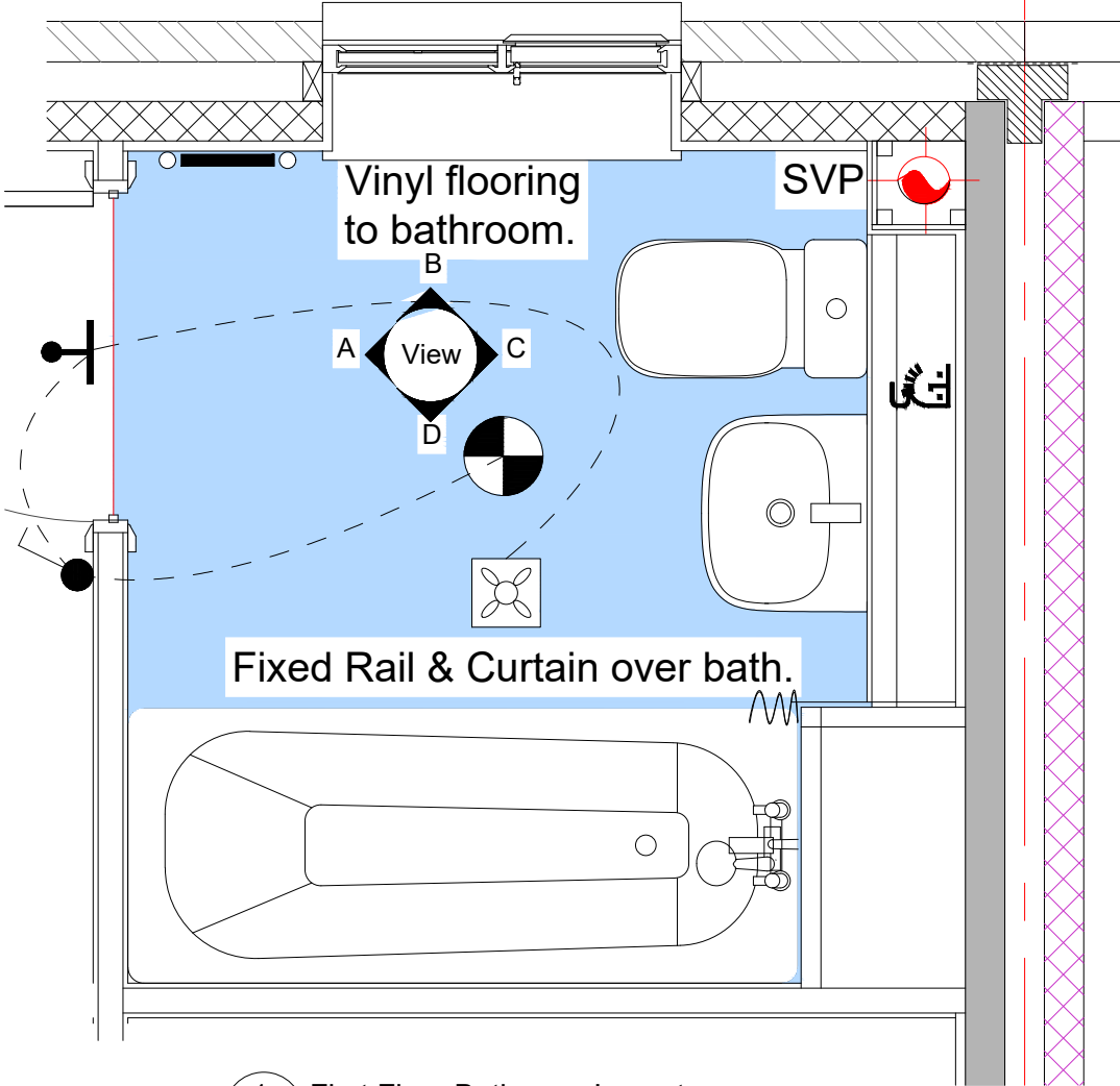
1 First Floor Bathroom Layout 1 : 20
