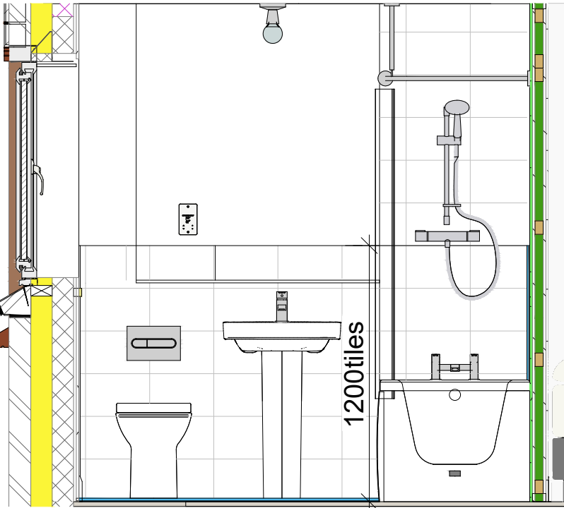
C Bathroom - View C 1 : 25
