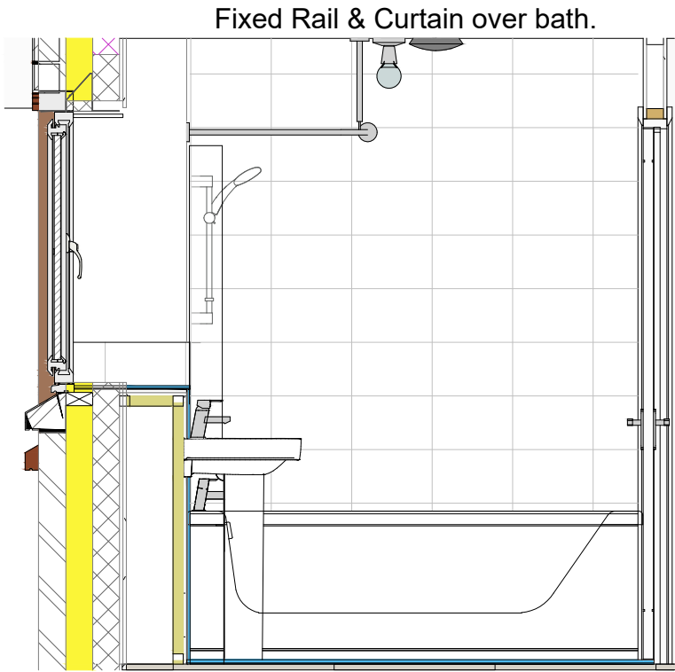
D Bathroom - View D 1 : 25
