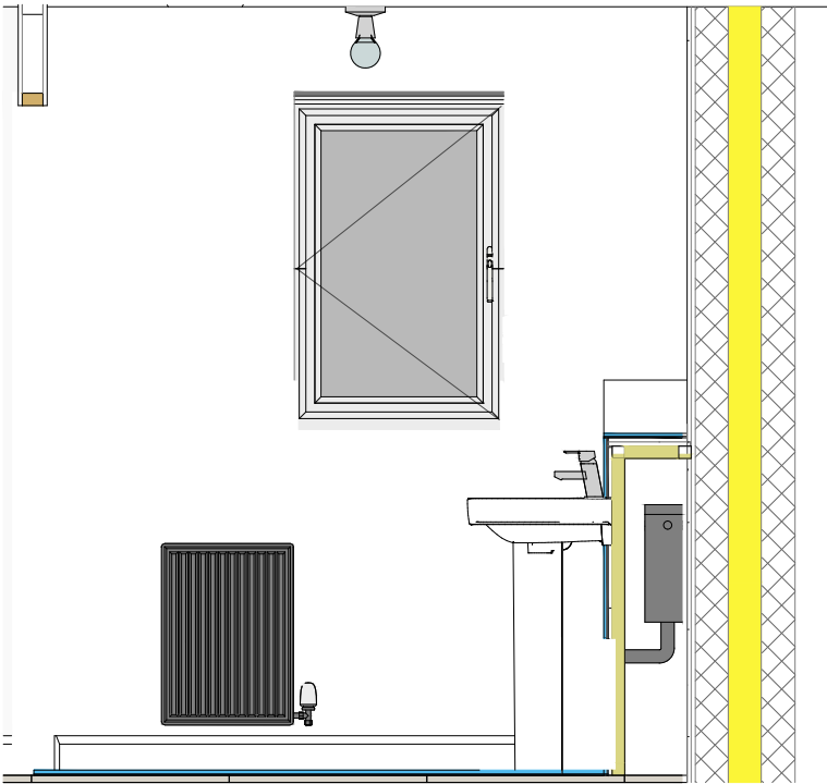
B Bathroom - View B 1 : 25
